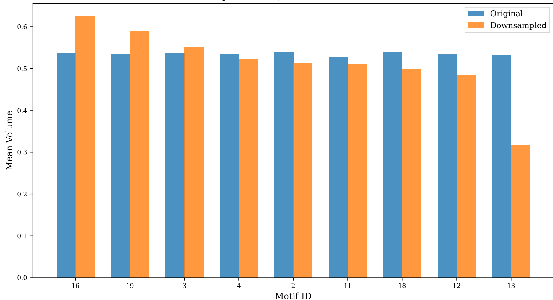
Mean Volume per Motif: Original vs Downsampled (sorted by downsampled) sigma: (1, 1) | volume: (0.03, 0.9)
